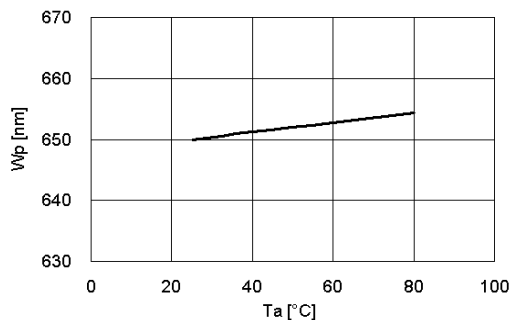
Fig.5 – Peak Wavelength (@10mA) vs. Ambient Temperature
