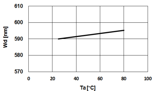
Fig.5 – Dominant Wavelength (@250mA) vs. Ambient Temperature
