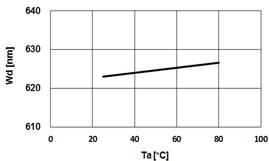
Fig.5 – Dominant Wavelength (@350mA) vs. Ambient Temperature
