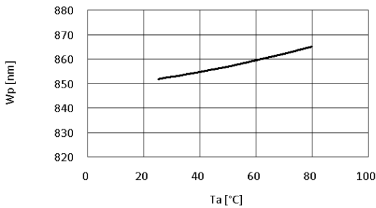
Fig.5 – Peak Wavelength (@100mA) vs. Ambient Temperature
