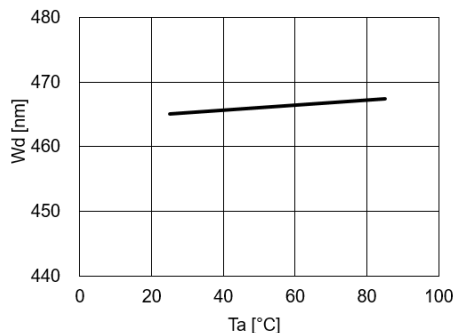
Fig.5 – Dominant Wavelength (@5mA) vs. Ambient Temperature
