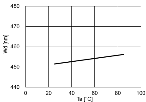
Fig.5 – Dominant Wavelength (@5mA) vs. Ambient Temperature
